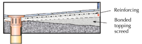
Figure 3. Tile bedding is drained. The membrane acts as a slip sheet, so a reinforced screed is required.
